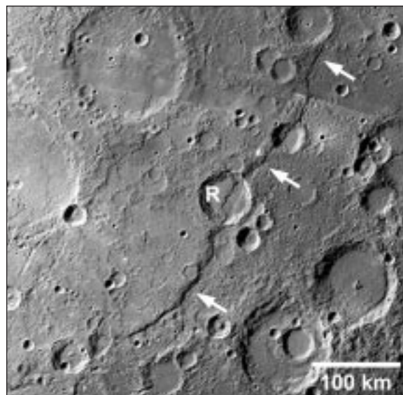
Figure 1. Mariner 10 mosaic of Discovery Rupes, largest known lobate scarp on Mercury (indicated by arrows). This scarp is ~550 km long and transects 60-km-diameter Rameau crater (R), and smaller 40-km-diameter crater to northeast. Scarp clearly deforms walls and offsets floor materials of two craters.
